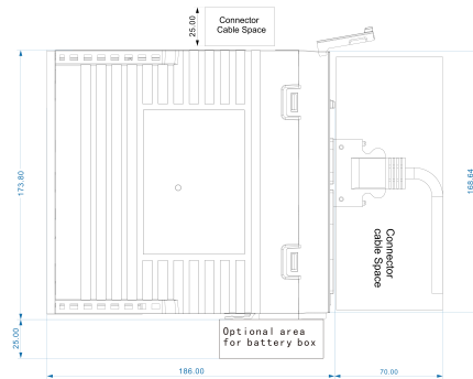
Mechanical View 2
