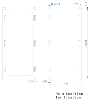
Mechanical View 1
