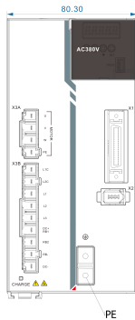
Mechanical View 3
