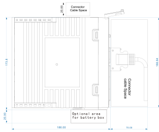
Mechanical View 1
