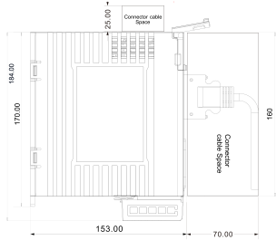
Mechanical View 1
