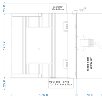
Mechanical View 1
