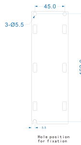
Mechanical View 2
