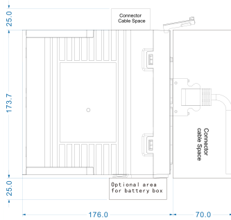
Mechanical View 1
