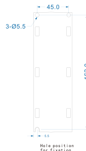
Mechanical View 2
