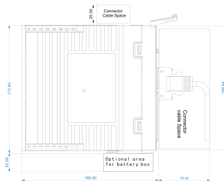
Mechanical View 1
