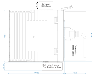
Mechanical View 1
