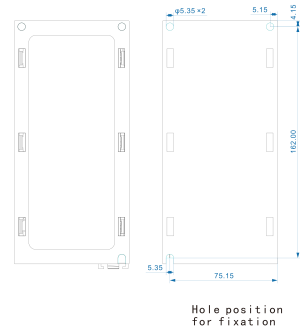
Mechanical View 2
