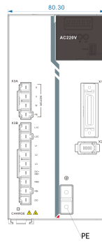
Mechanical View 3
