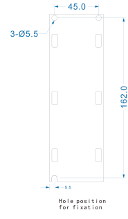
Mechanical View 3
