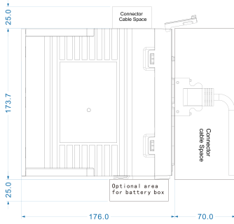
Mechanical View 1
