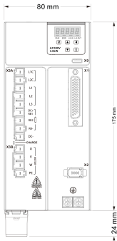
Mechanical View 4
