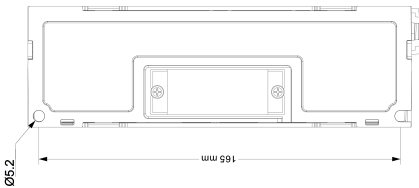
Mechanical View 3
