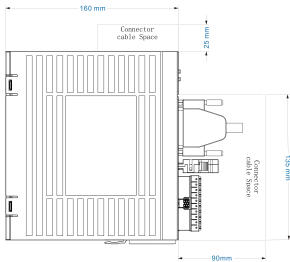
Mechanical View 3
