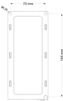
Mechanical View 3
