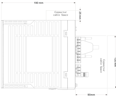
Mechanical View 1
