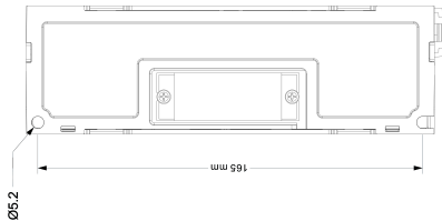
Mechanical View 4
