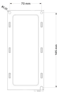
Mechanical View 3
