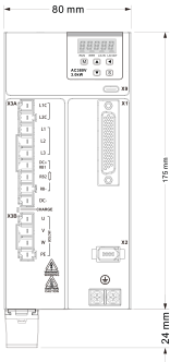
Mechanical View 4
