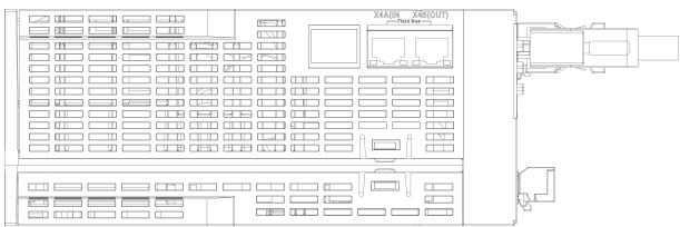
Power Connector Pinout
