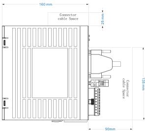
Mechanical View 3
