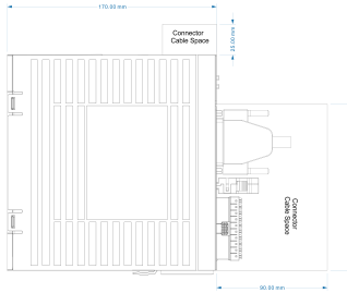
Mechanical View 1
