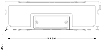
Mechanical View 3
