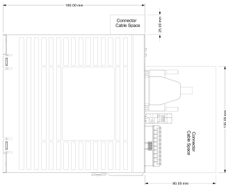
Mechanical View 1
