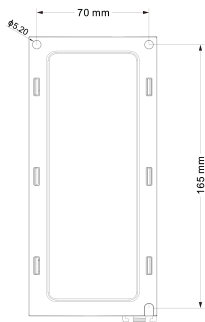
Mechanical View 3
