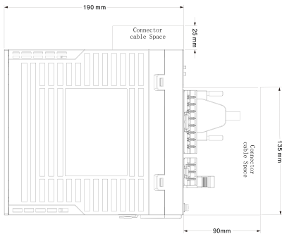
Mechanical View 1
