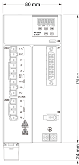
Mechanical View 4
