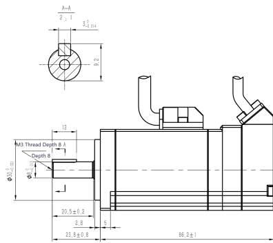
Mechanical View 1
