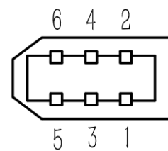
Feedback Connector Pinout
