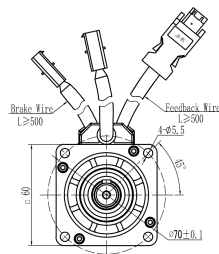
Mechanical View 4
