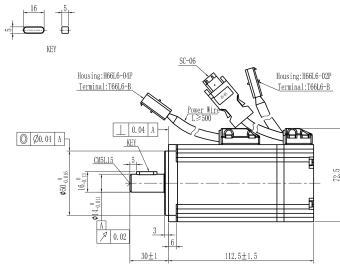
Mechanical View 1
