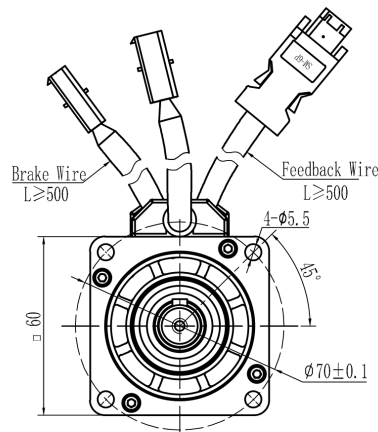
Mechanical View 2
