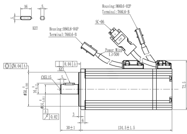
Mechanical View 1
