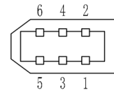
Power Connector Pinout
