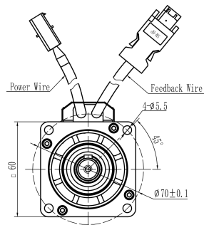
Mechanical View 3
