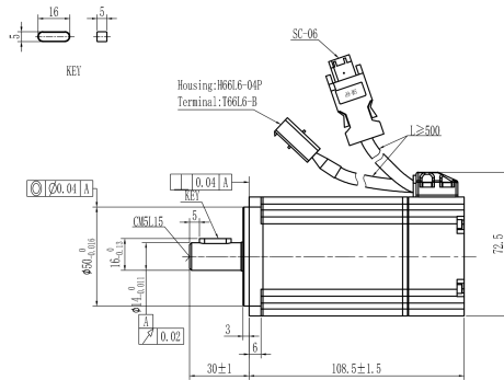
Mechanical View 1
