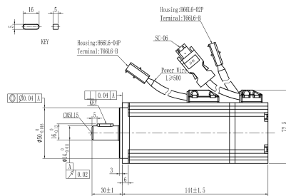
Mechanical View 1
