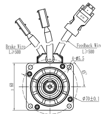
Mechanical View 4
