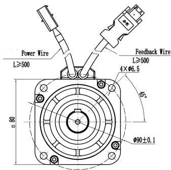
Mechanical View 3
