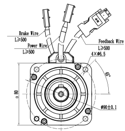
Mechanical View 5
