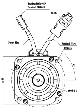
Mechanical View 1
