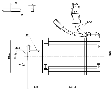
Mechanical View 3
