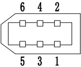
Power Connector Pinout
