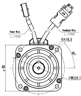
Mechanical View 3
