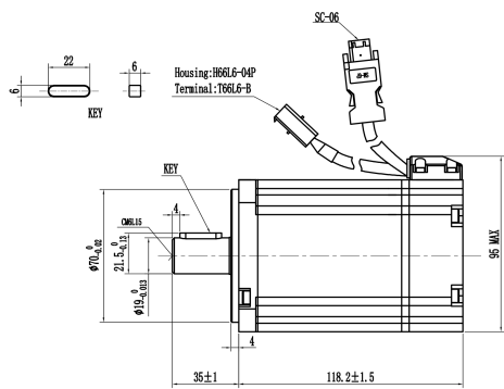
Mechanical View 1
