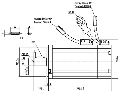
Mechanical View 1
