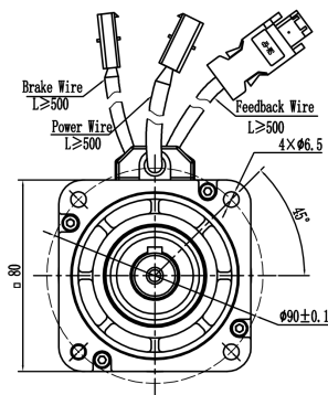
Mechanical View 3
