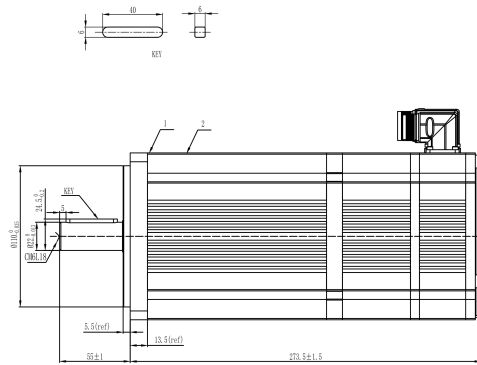
Mechanical View 1
