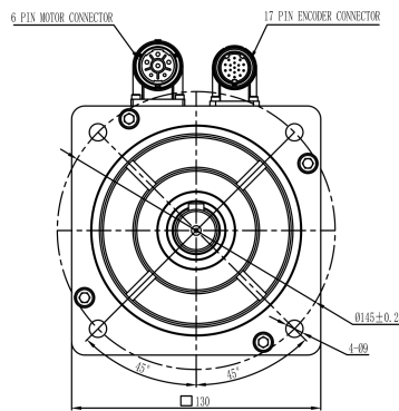
Mechanical View 3
