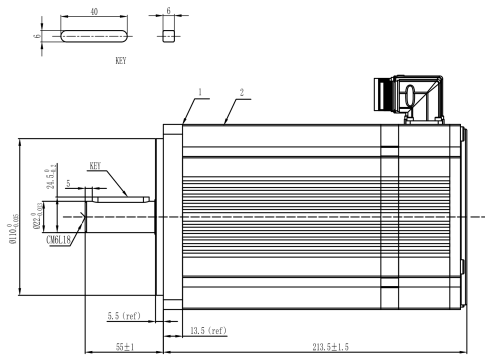
Mechanical View 1
