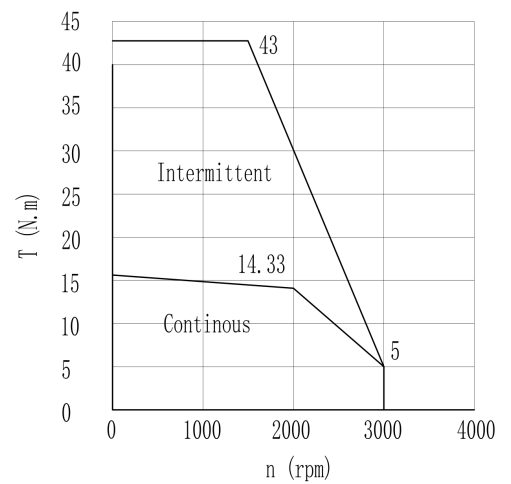
Torque-Speed Curve
