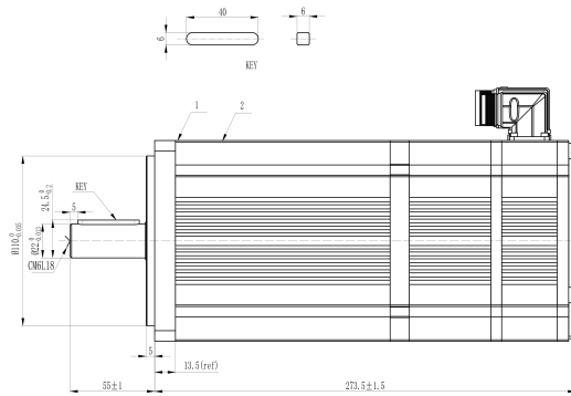
Mechanical View 1
