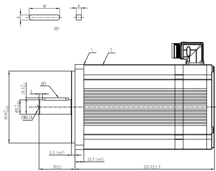
Mechanical View 1
