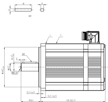
Mechanical View 1
