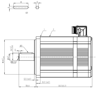
Mechanical View 1
