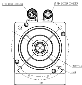
Mechanical View 3
