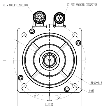
Mechanical View 3
