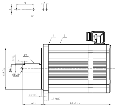
Mechanical View 1
