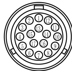
Mechanical View 2
