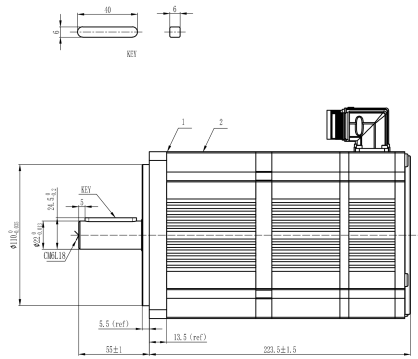
Mechanical View 2
