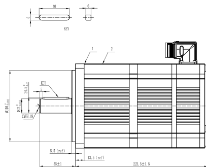
Mechanical View 1
