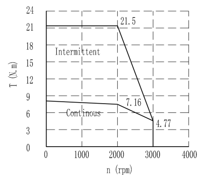
Torque-Speed Curve
