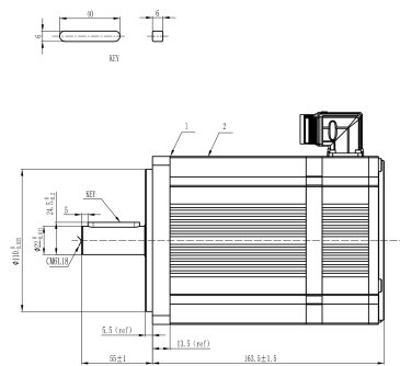
Mechanical View 1
