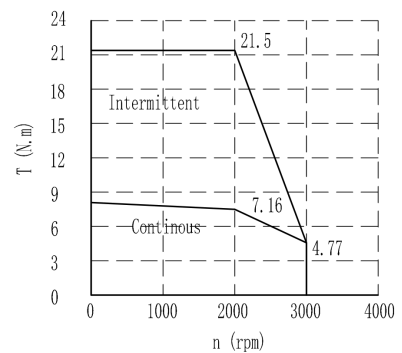
Torque-Speed Curve
