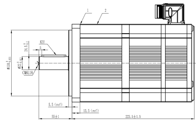
Mechanical View 4
