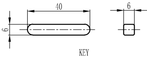
Mechanical View 1
