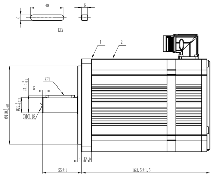
Mechanical View 1
