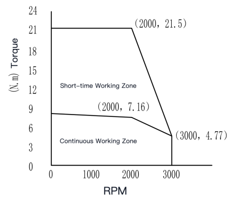
Torque-Speed Curve
