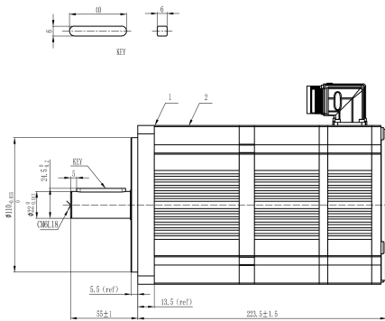
Mechanical View 1
