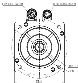
Mechanical View 3
