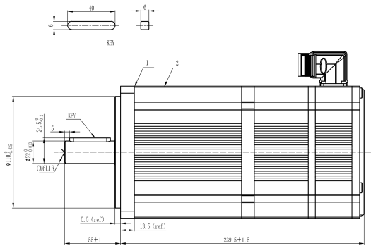
Mechanical View 1
