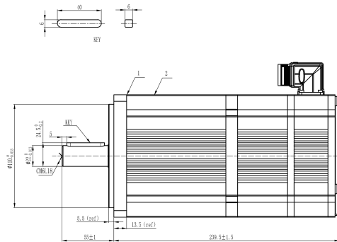
Mechanical View 1
