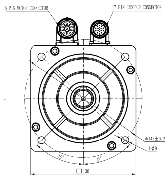
Mechanical View 3
