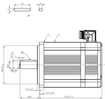
Mechanical View 1
