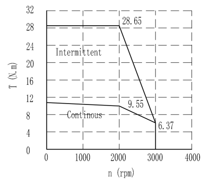
Torque-Speed Curve
